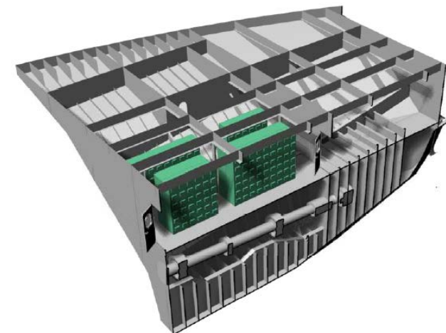
Figure 32: Battery Room Arrangement Profile View – Spear SMAR-3T
